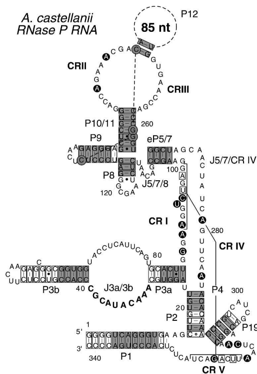
FIGURE 2. Secondary structure of A. castellanii RNase P RNA. Helices are labeled 5' to 3', P1–P19 as defined for bacterial RNase P RNA (Haas et al. 1994). Nucleotides circled in black are universally conserved among all three domains of life and constitute the five Conserved Regions I–V. Base pairs indicated by closed dots indicate a conserved noncanonical (G–U or A–C) interaction. The A. castellanii RNase P RNA secondary structure is based on evidence provided by an alignment of 63 diverse eucaryal RNase P RNA sequences. Shaded boxes indicate base pairs supported by a H_{ij} score \geq 32 ( \chi^2 test, P < 0.0002 ; 9 d.f.). Outlined base pairs indicate base pairs confirmed by covariation among eucaryal RNase P RNAs. Bold nucleotides indicate the location of the weak consensus sequence identified in J3a3b of eucaryal RNase P RNAs. Lines connecting circled bases indicate tertiary interactions supported by statistical covariation analysis. The structure of the P12 helix is not established by comparative results and so is represented by a dashed circle. The 5' and 3' ends of the A. castellanii RNase P RNA, as well as all new sequences in this study, have not been experimentally determined. Instead, the terminus of helix P1 is arbitrarily established as the end of complementarity.
